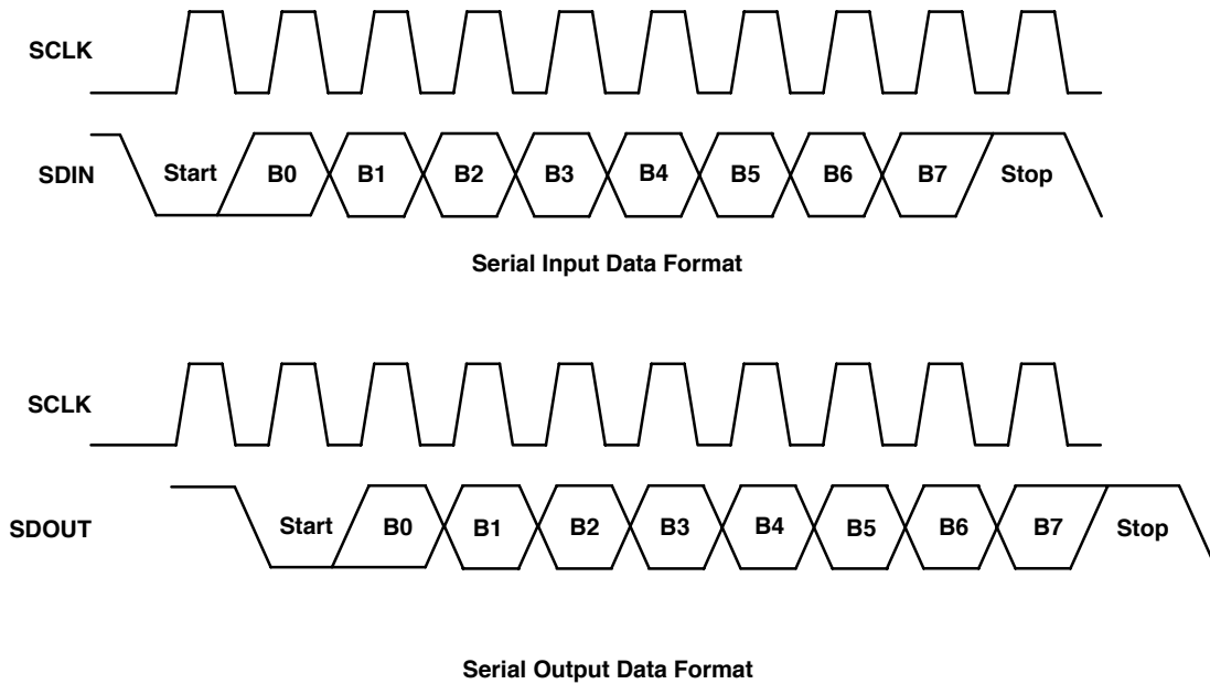
Figure 4. TSL3301 Serial I/O
