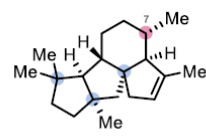
iso-phomopsene (3) revised structure (this work)
