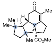
methyl phomopsenonate (2)
