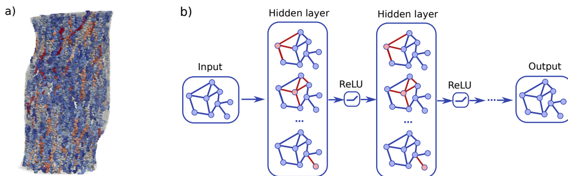
Figure 1: a) Clusters of grains forming force chains during triaxial compression of a digital specimen of sand simulated with the Level-set Discrete Element Method [1], b) Architecture of a graph neural network.
