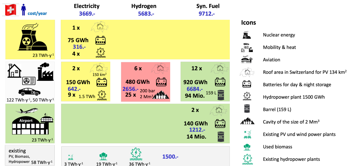
Fig. 3 The three energy systems presented for the complete substitution of fossil fuels with renewable energy. The PV surface area is shown as the roof area in Switzerland. The battery represents the local day/night storage and the seasonal storage as compared to Grande Dixence storage lake, the volume of the Gotthard base tunnel, and barrels of oil. 19 The total annual cost of energy per capita is indicated on top; currently the energy cost per capita amounts to 3000.-/year.
