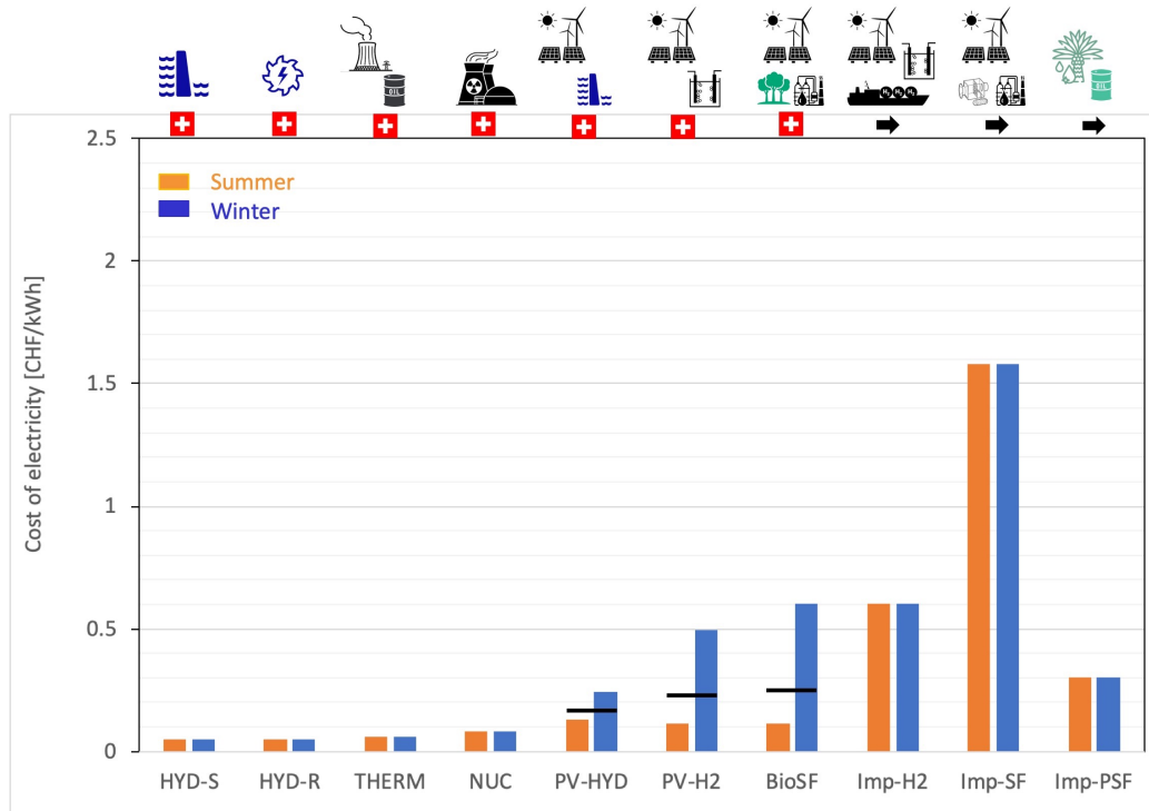
Fig. 7b Production cost of the electricity (without grid cost per kWh without orange and with blue seasonal storage for the 3 winter months. Bars in bold color represent the future cost (PV 400 CHF/kW p , Battery 50 CHF/kWh, electrolyzer 500 CHF/kW, efficiency 90%). The average cost is composed of 75% cost without seasonal storage and 25% cost with seasonal storage, solid line for future average cost (—).
