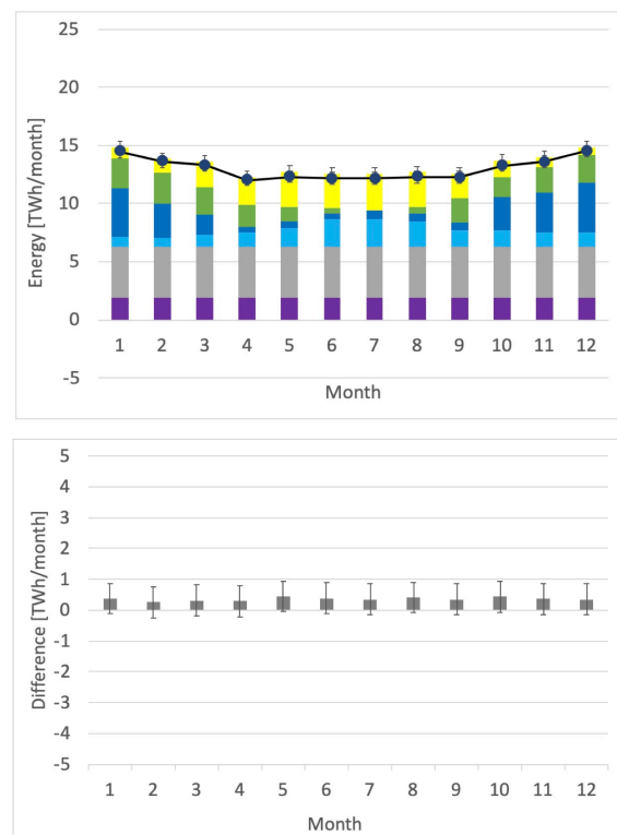
Fig. 6b Electrified Swiss energy system (based on 2019) with the contributions from the different sources of energy: ■ Photovoltaic, ■ Biomass, ■ Storage hydropower, ■ River hydropower, ■ 6 Power Plants Unit's (PPU's), ■ Aviation fuel (CO 2 neutral). The energy demand is shown by the black markers and line, energy demand 156 TWh·y -1 .
