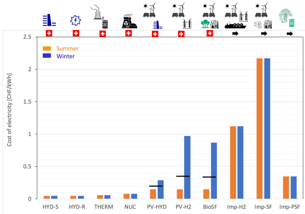
Fig. 7a Production cost of the electricity (without grid cost per kWh without ■ and with ■ seasonal storage for the 3 winter months. Bars represent the cost today. The average cost (—) is composed of 75% cost without seasonal storage and 25% cost with seasonal storage, solid line for current average cost.
