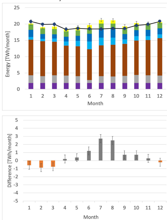
Fig. 6a Current Swiss energy system (2019) with contributions from the different sources of energy: ■ Photovoltaic, ■ Biomass, ■ Storage hydropower, ■ River hydropower, ■ Fossil fuel, ■ Nuclear power plants, ■ Aviation fuels. The energy demand is shown by the black markers and line, energy demand 232 TWh·y -1 .
