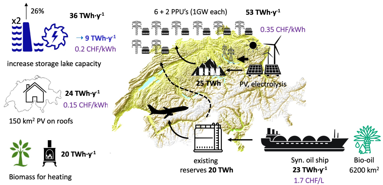
Graphical abstract: Future supply of Switzerland with renewable energy. Assuming the volume of the hydroelectric storage lakes is doubled, the roof area is covered with photovoltaics, and eight power plant units are able to produce 1 GW on demand and are fueled with hydrogen or bio-oil. The reserves are the existing oil tanks, and the bio-oil is also used for aviation. Bio-oil can be produced in abundant places, e.g., Australia or Africa, where palm oil plantations are installed.
