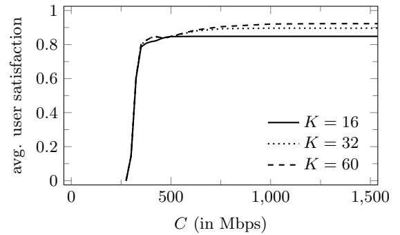
Figure 9: Average user satisfaction vs. CDN capacity C .
