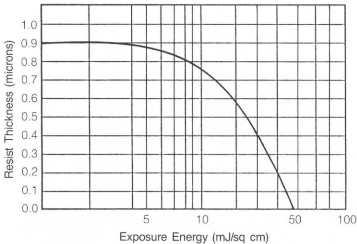
CHARACTERISTIC CURVE
